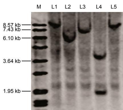
Fig. 7 Southern blot analysis of transgenic soybeans
